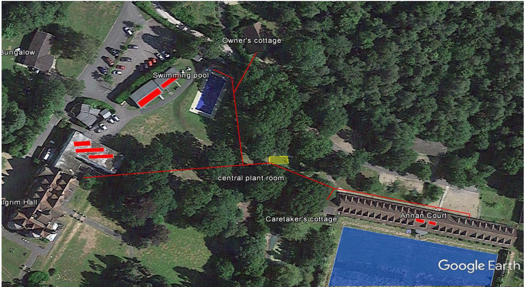
Site layout with DH pipes Rev2
